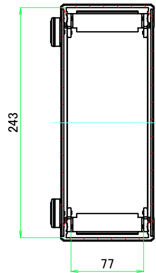
B-B (1:4)
